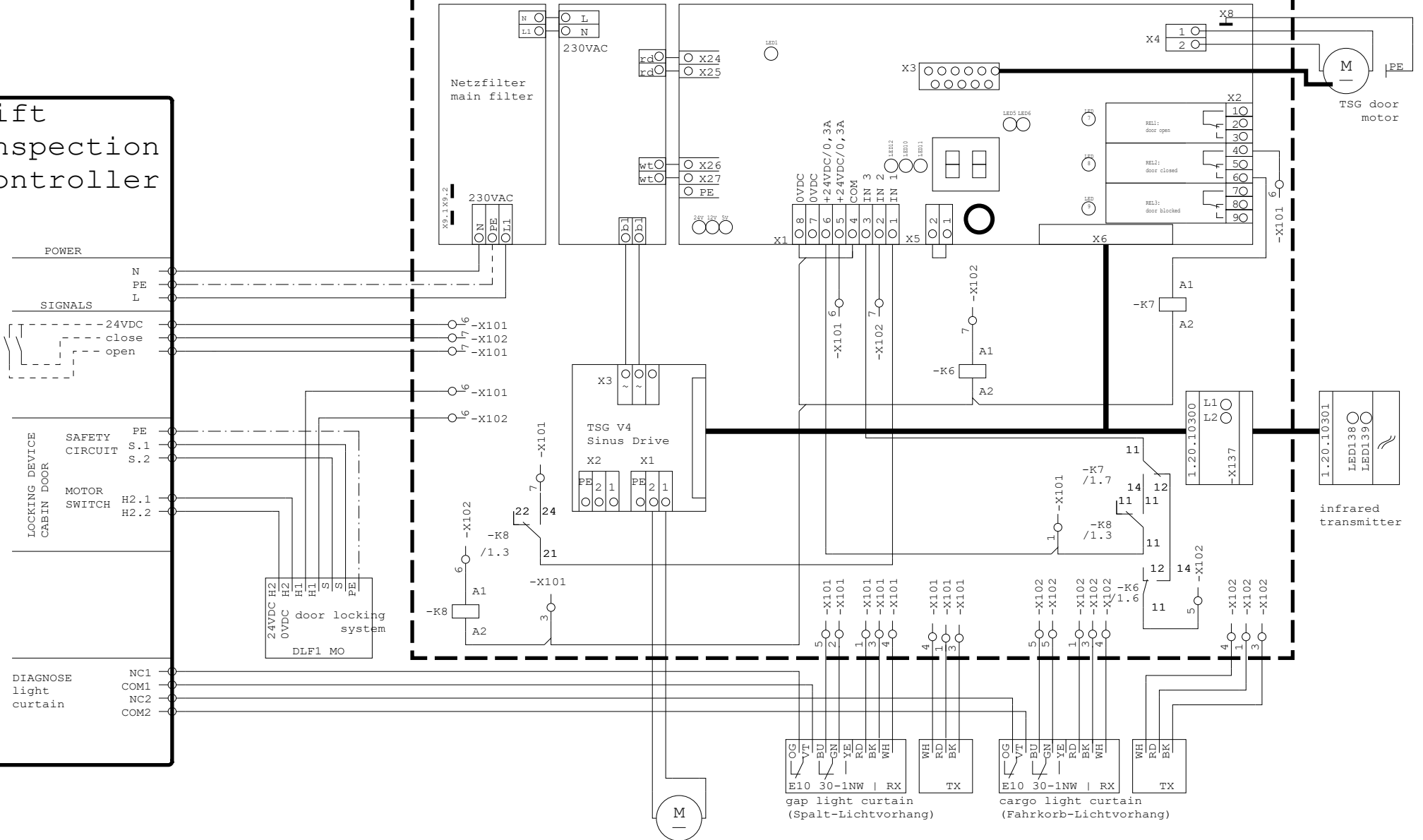
TSG Sinus Drive for moving interlock shaft door
